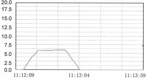
3 RIGHT SEAL TEST
